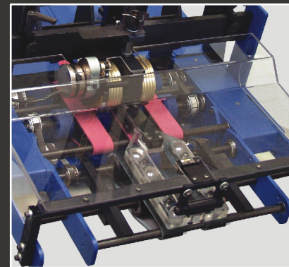
►► Available on the Packaging Series for Guaranteed Sheet Separation. This feature is required for precise counting and single shot feed on demand applications
