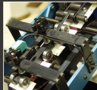
►► The accelerator extension creates a perfect separation for single shot or batch counting
