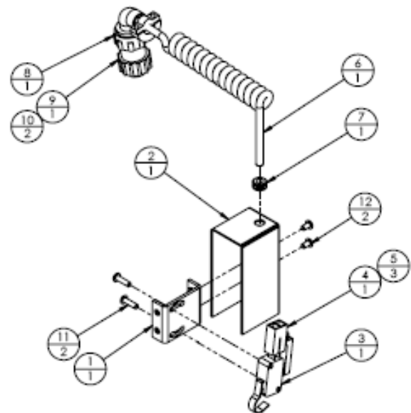
ASSY, LOW PRODUCT SWITCH
